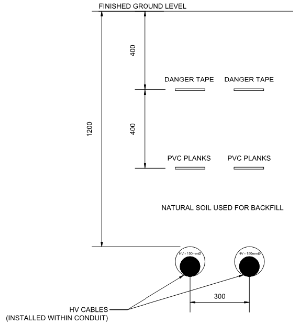
HV Cable Route – Installed within Conduit/Polypipe
