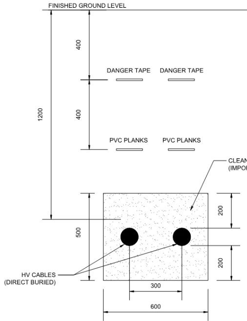
HV Cable Route – Direct Buried
